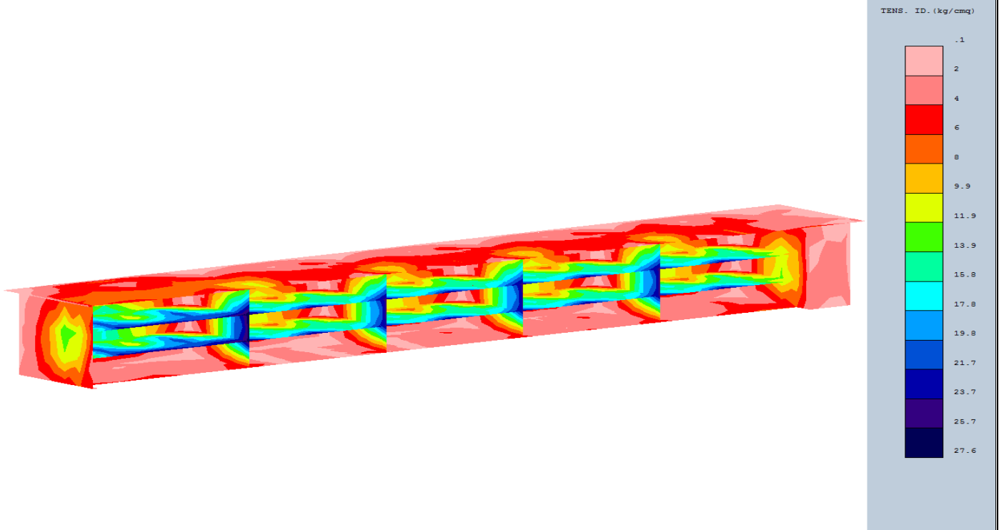
1 - TENS. ID. COMBINAZ.N. 5
