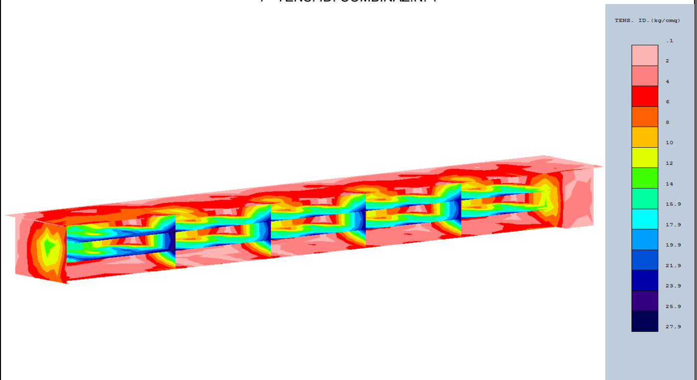
1 - TENS. ID. COMBINAZ.N. 1
